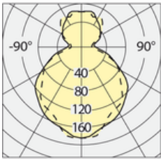
cd/klm FLUODimmable
