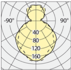
cd/klm Designers
